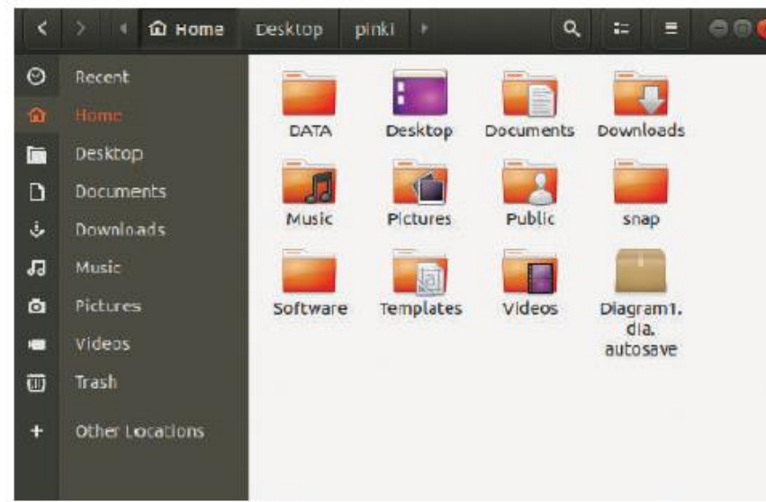
Figure 3.18: File Explorer
